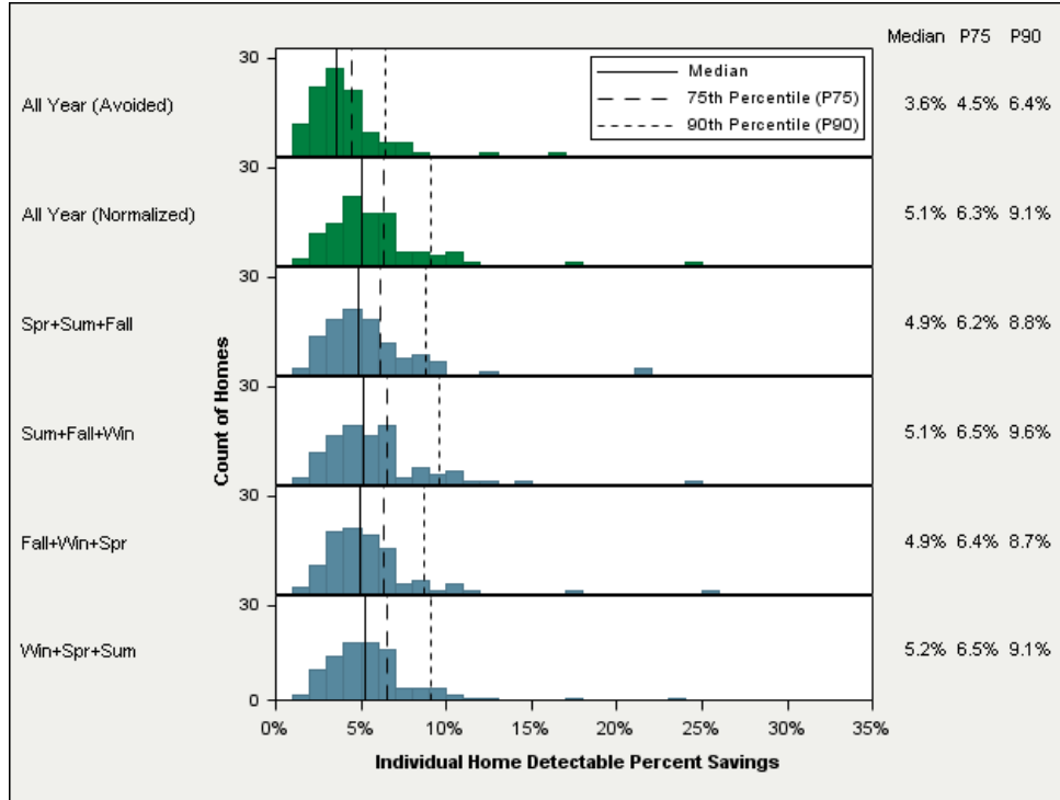
Figure 12. Detectable Percent Savings for Nine-Month Models
