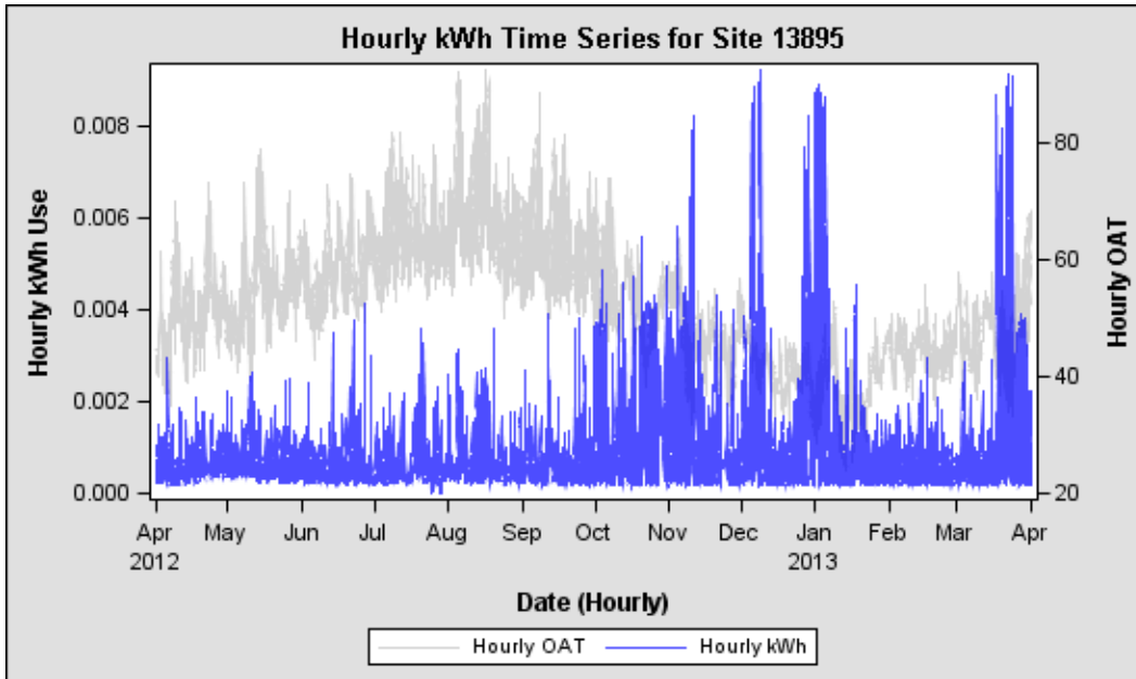
Figure 3 . Example Time-Series Chart for Home with High Detectable Percent Savings
