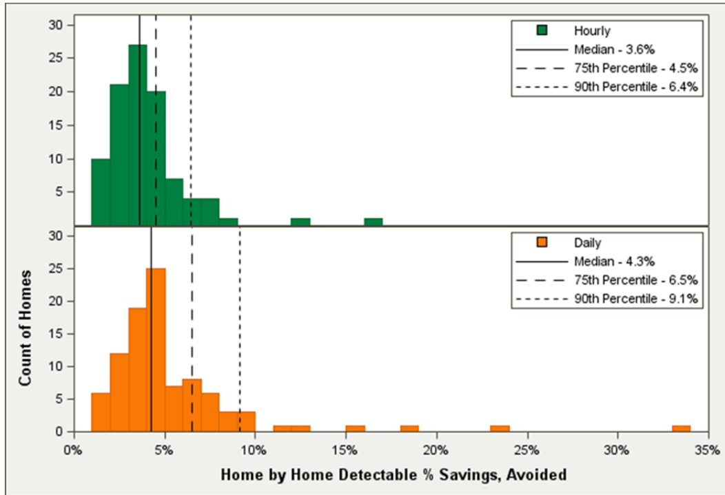
Figure 4. Detectable Percent Savings for Hourly and Daily Models at 90 % Confidence Level
