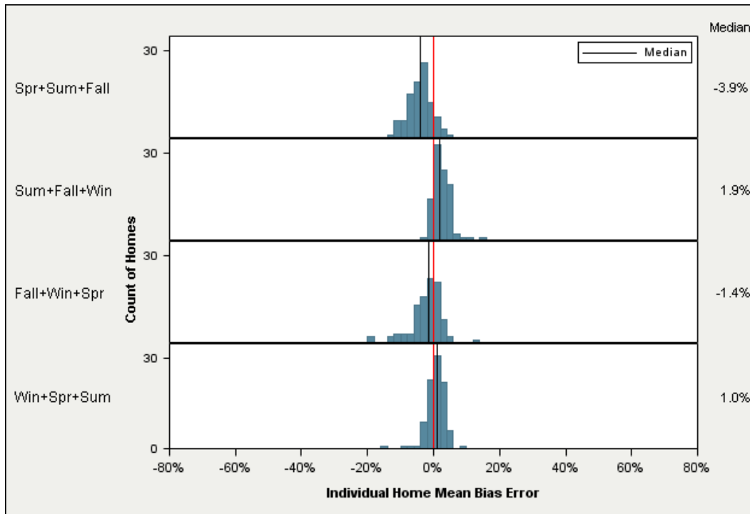
Figure 8. Mean Bias Errors for Nine-Month Models
