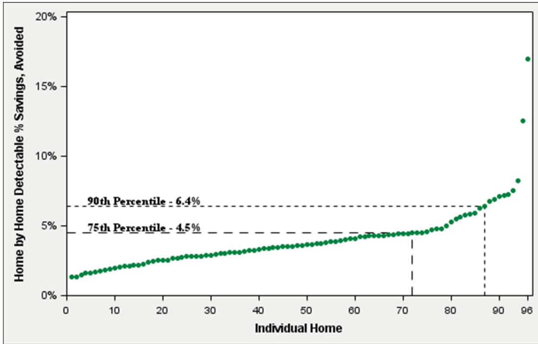
Figure 2. Detectable Percent Savings for Each Home in the Study Dataset (90% Confidence Level)
