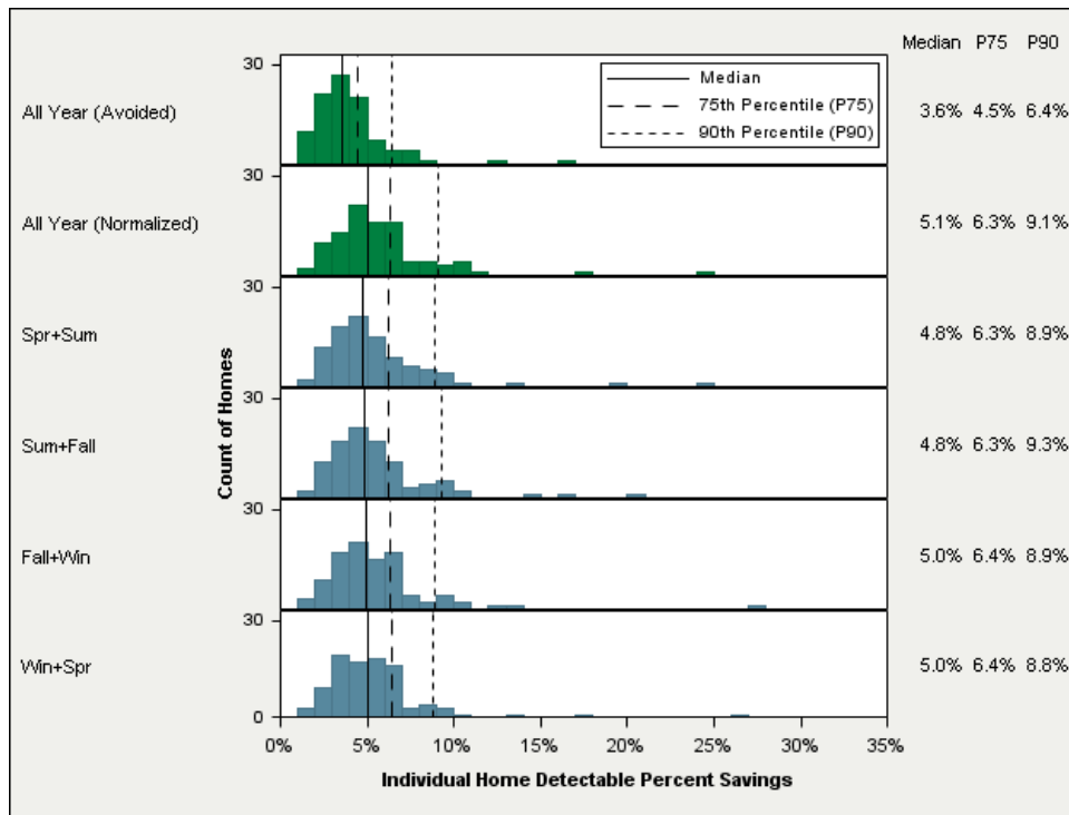
Figure 11. Detectable Percent Savings for Six-Month Models
