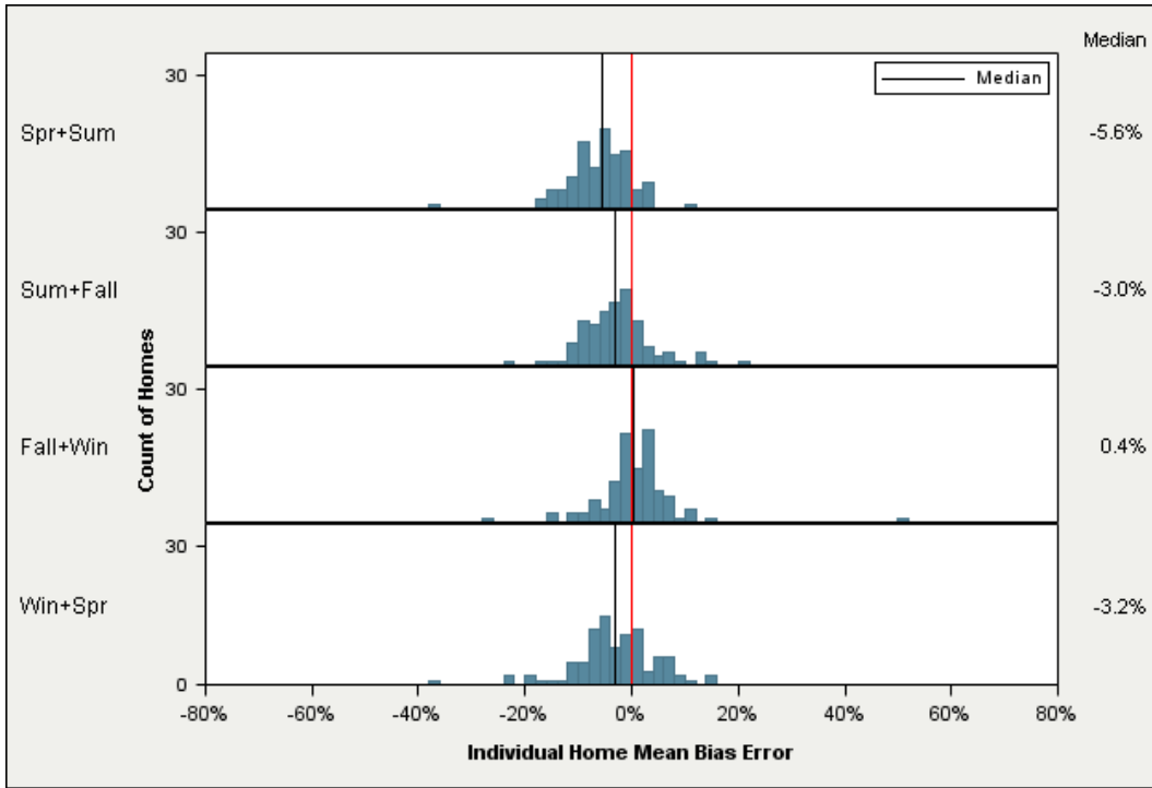
Figure 7. Mean Bias Errors for Six-Month Models
