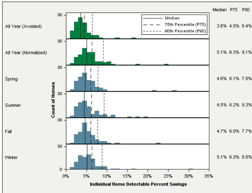
Figure 10. Detectable Percent Savings for Three-Month Models
