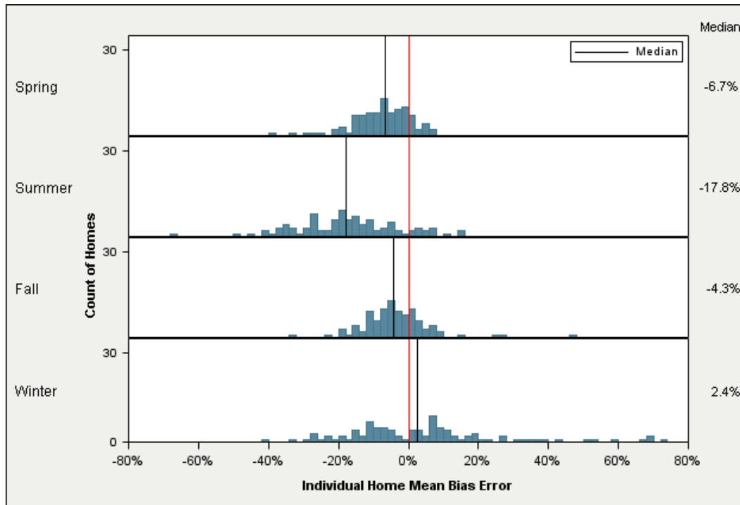
Figure 6. Mean Bias Errors for Three-Month Models
