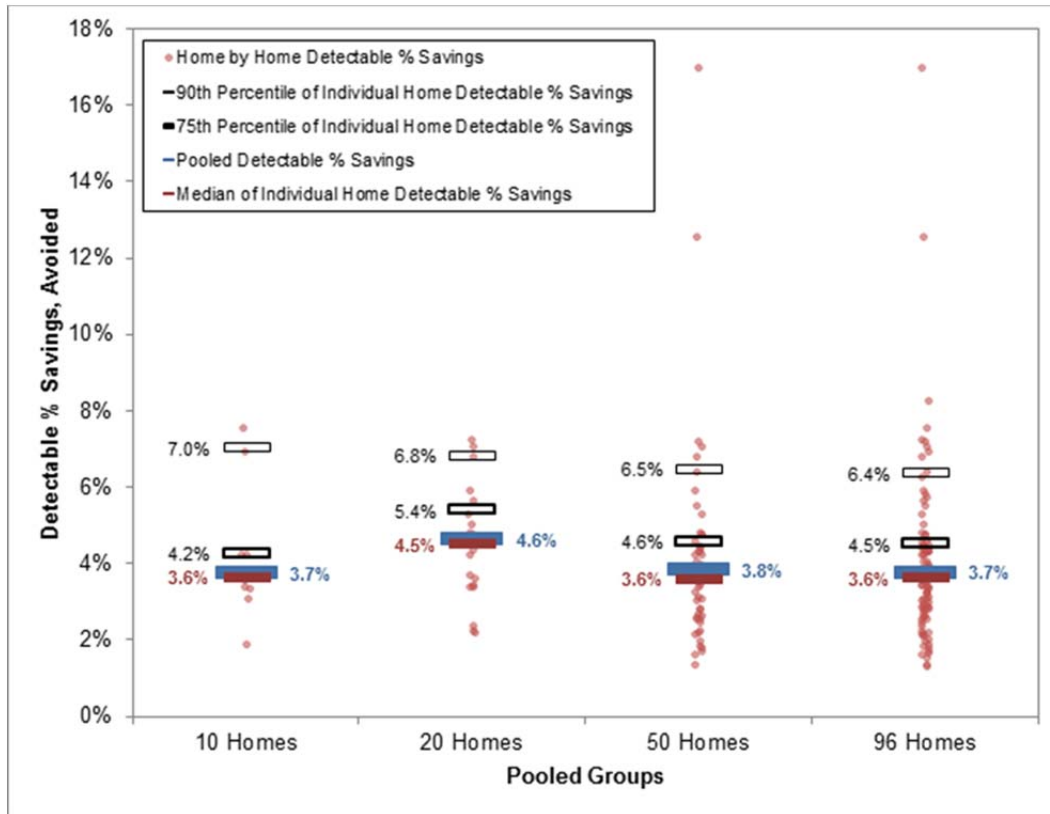
Figure 9. Pooled Baseline Modeling Results
