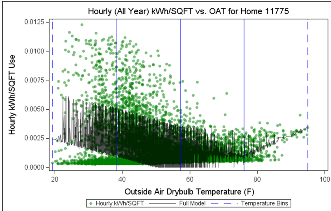
Figure 1. Example Data from a Home in the RBSA Dataset, Showing Hourly Energy Consumption Values and the Baseline Regression Developed Under This Project
