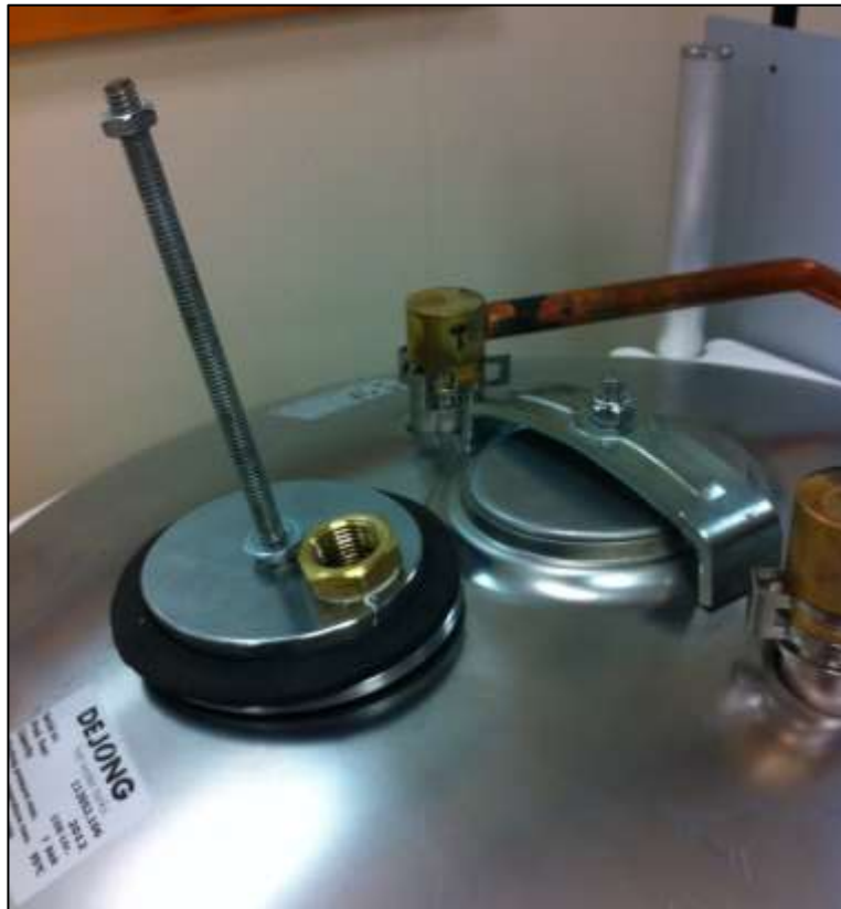
Figure 3. Custom Lid for Thermocouple Tree Access
