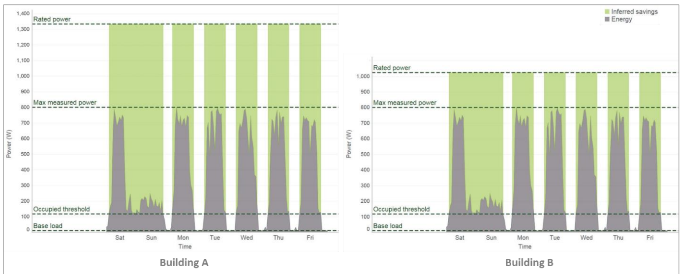
Figure 11. Example of two buildings with the exact same lighting load profile after all the controls implemented.
