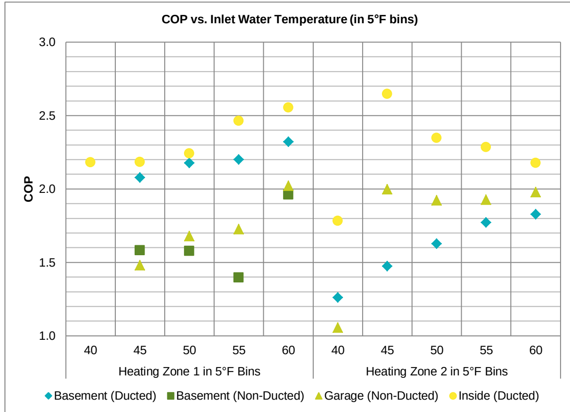
Figure 18 - COP vs. Inlet Water Temperature (in 5° F bins)
